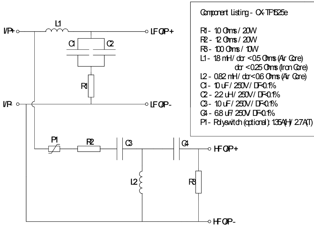
Crossover Schematic: CX-TF1525e
