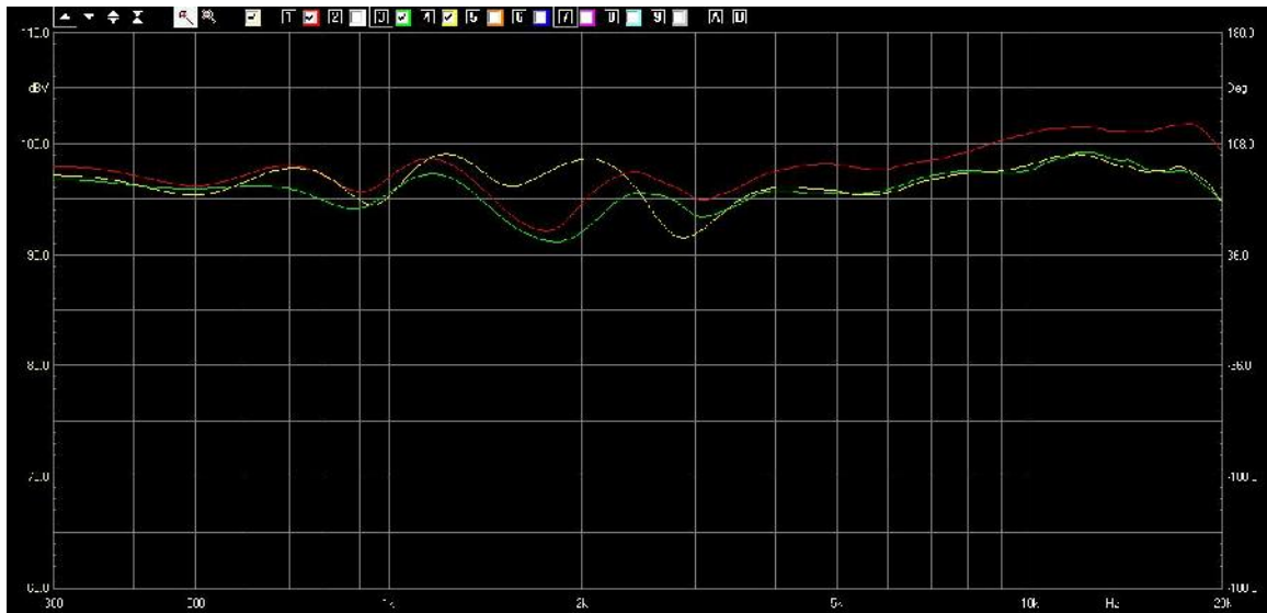
Vertical Dispersion: on-axis(red), +10deg(green), -10deg(yellow) (1m measurements normalized to 2.83V)
