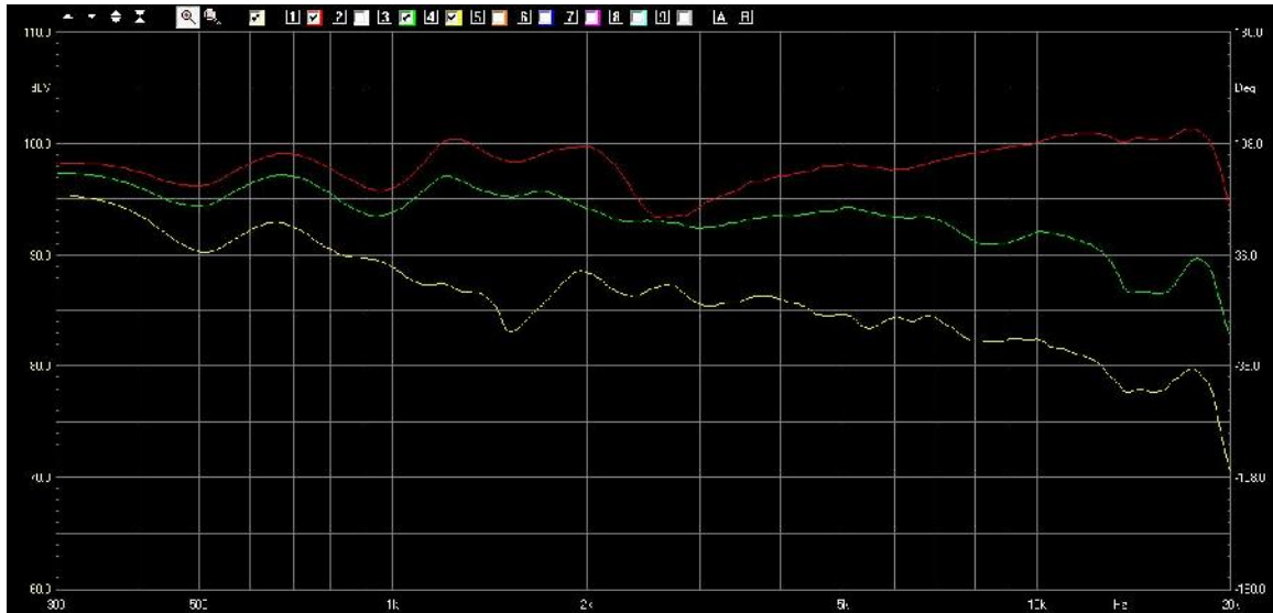
Horizontal Dispersion: on-axis(red), 30(deg), 60deg(yellow) (2m measurements normalized to 2.83V/1m)
